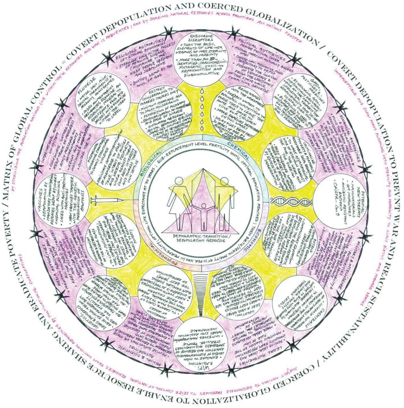
Figure 1: The depopulation/globalization system model.
