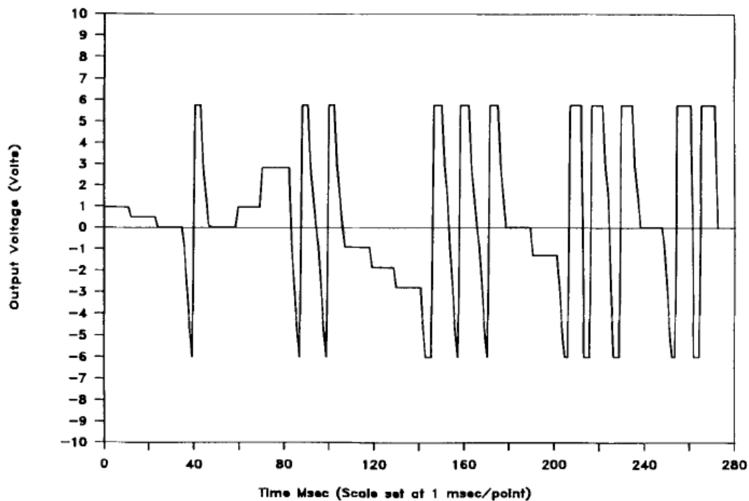
Figure 1: The burst-firing pattern that was generated by converting a series of preprogrammed successive numbers by a computer software to voltage (y-axis). In our study the point durations were 3 ms.
